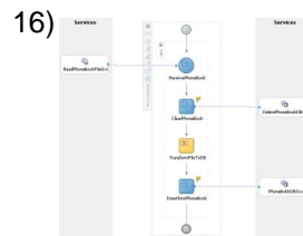
batch processing
