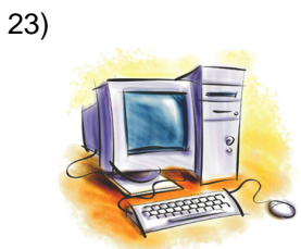
computation
