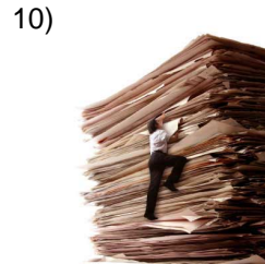
shared file
