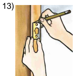
to install
